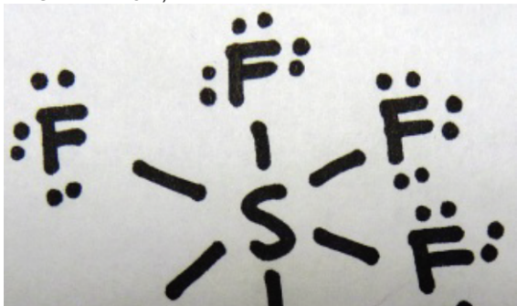
Photo 19: SF 6 Lewis Structure and VSEPR Model (SAMPLE ANSWER BELOW)
