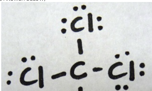
Photo 3: \text{CCl}_4 Lewis Structure and VSEPR Model (SAMPLE ANSWER BELOW)
