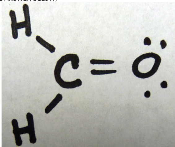
Photo 9: CH 2 O Lewis Structure and VSEPR Model (SAMPLE ANSWER BELOW)
