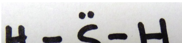
Photo 18: H 2 S Lewis Structure and VSEPR Model (SAMPLE ANSWER BELOW)
